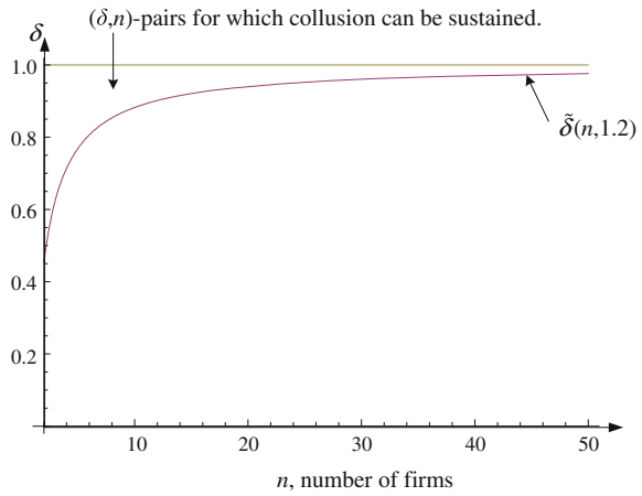
Fig. 6.5 Critical threshold
